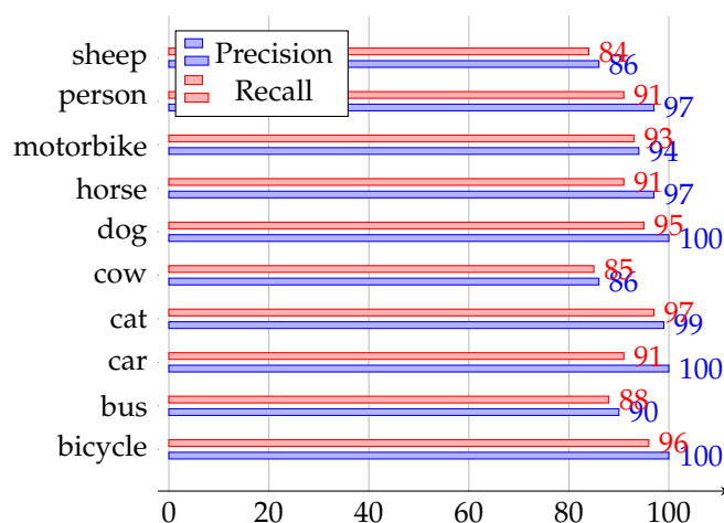
Figure 13. Experiment 2—Efficiency of the PASCAL dataset (see Table 14).
